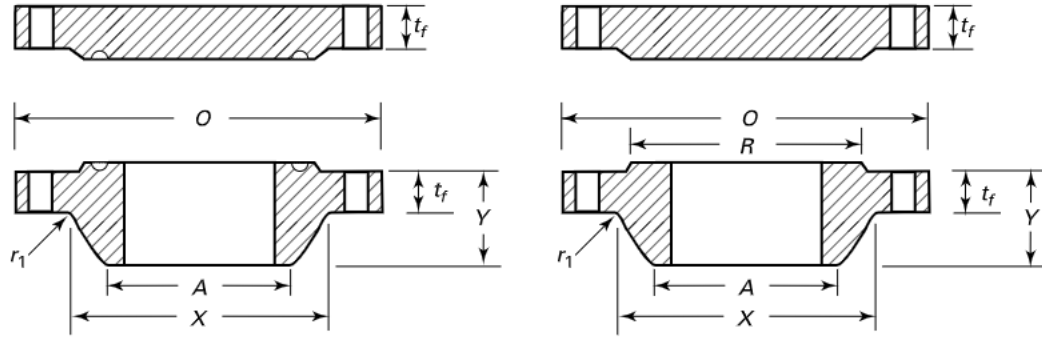
Ring Joint
